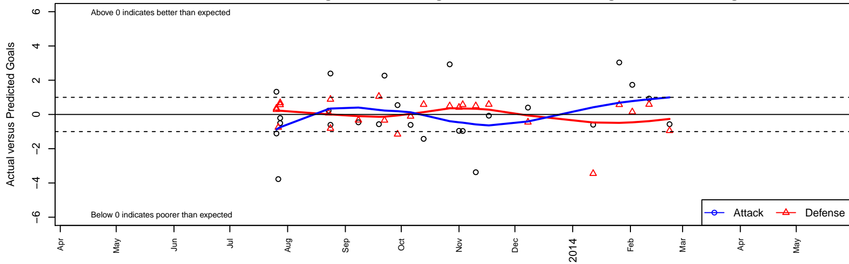
Crossfire Select Jinneman B95 Dots are actual minus expected GF (blue circles) and GA (red triangles). Blue line is smoothed change in attack strength. Red is smoothed change in defense strength.
